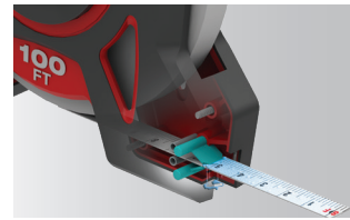
GRIME GUARD™ Industry's First Blade Wiper
